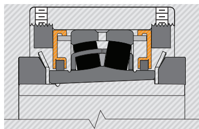
TAA/DAA – Double Nut Tapered Adapter Lock
